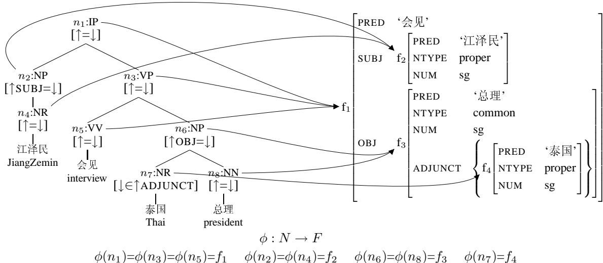
Figure 1: C- and f-structures with \phi links for the sentence “江泽民会见泰国总理”
