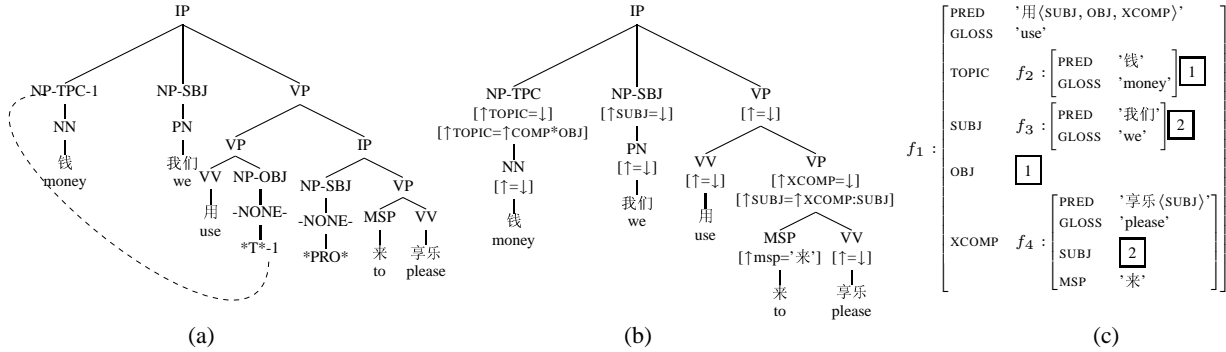
Figure 2: (a) the CTB tree; (b) LFG c-structure with functional equations; (c) corresponding f-structure. ( \uparrow ) in the functional annotation refers to the f-structure associated with the mother node and ( \downarrow ) to that of the local node.
