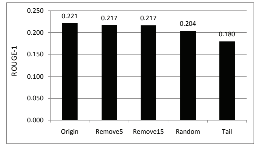
Figure 10: The impact of the search engine, on Wikipedia test set using ROUGE-1 performance.
