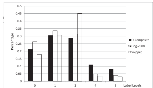
Figure 8: Label level distributions of systems on TREC 2009 data set.
