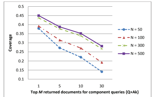
Figure 5: The average coverage of the top returned search documents of the original queries \{Q\} over the top returned documents of the component queries \{Q + A_k\} .
