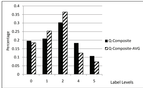
Figure 9: Label level distributions of Q-Composite and Q-Composite-AVG on TREC 2009 data set.
